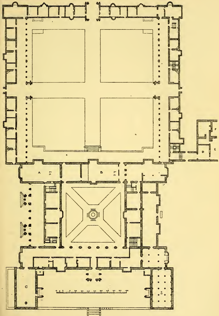
AUDLEY END, ESSEX. (SOANE COLLECTION.)
